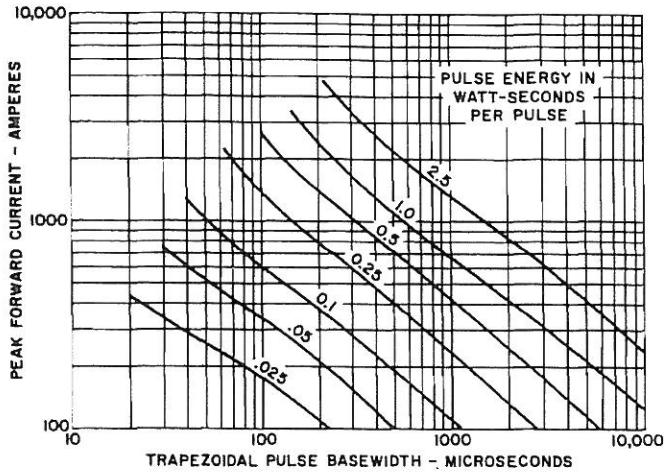
7. TRAPEZOIDAL PULSE ENERGY DI/DT (RISING & FALLING) = 100 A/μs ( T_J = 175^\circ\text{C} )
