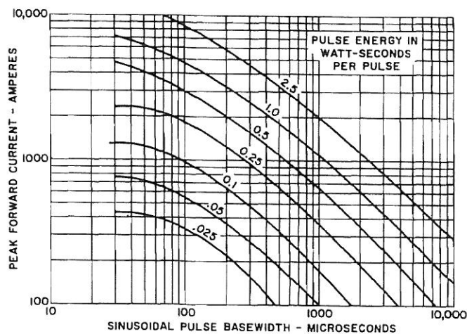
4. SINUSOIDAL PULSE ENERGY ( T_J = 175^\circ\text{C} )
