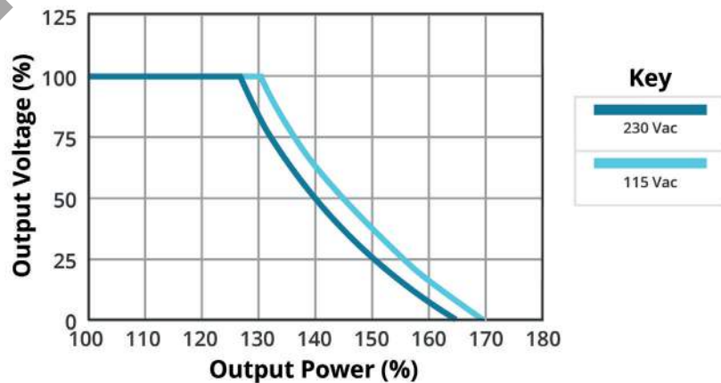
TYPICAL OVER CURRENT PROTECTION CURVE (PDRC-36-24)
