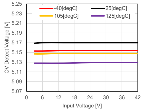
V OVSET = 5.17V
