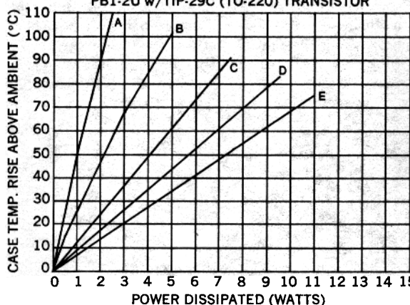
PB1-2U w/TIP-29C (TO-220) TRANSISTOR
