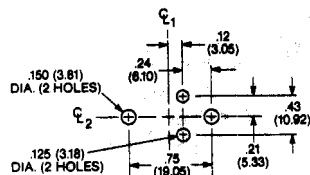
-3 HOLE PATTERN
