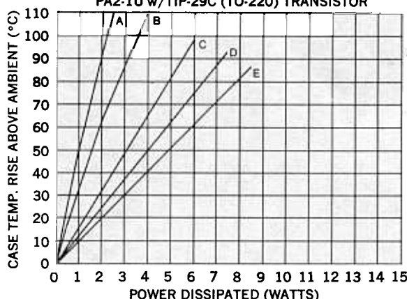
PA2-1U w/TIP-29C (TO-220) TRANSISTOR
