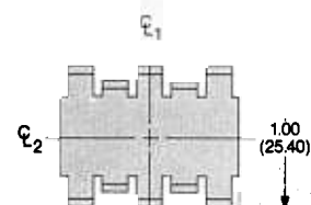
-1 HOLE PATTERN
