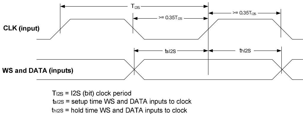
Figure 7-2. I2S input timing in audio slave mode (I2SCNF_IN[7]=0)
