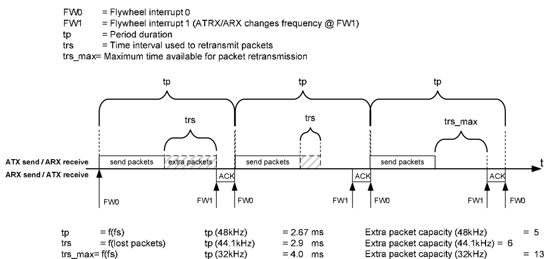
Figure 4-3 nRF24Z1 data streaming principle
