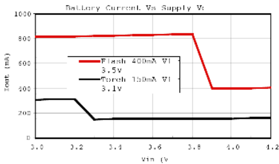
Fig. 16: Battery Current vs Supply Voltage D1=AOT2015HPW-1915 LED, R_{SENSE}=0.3\Omega R_{SET}=106k\Omega , C_{IN}=2.2\mu F , C_{FC}=0.47\mu F , C_{OUT}=1\mu F
