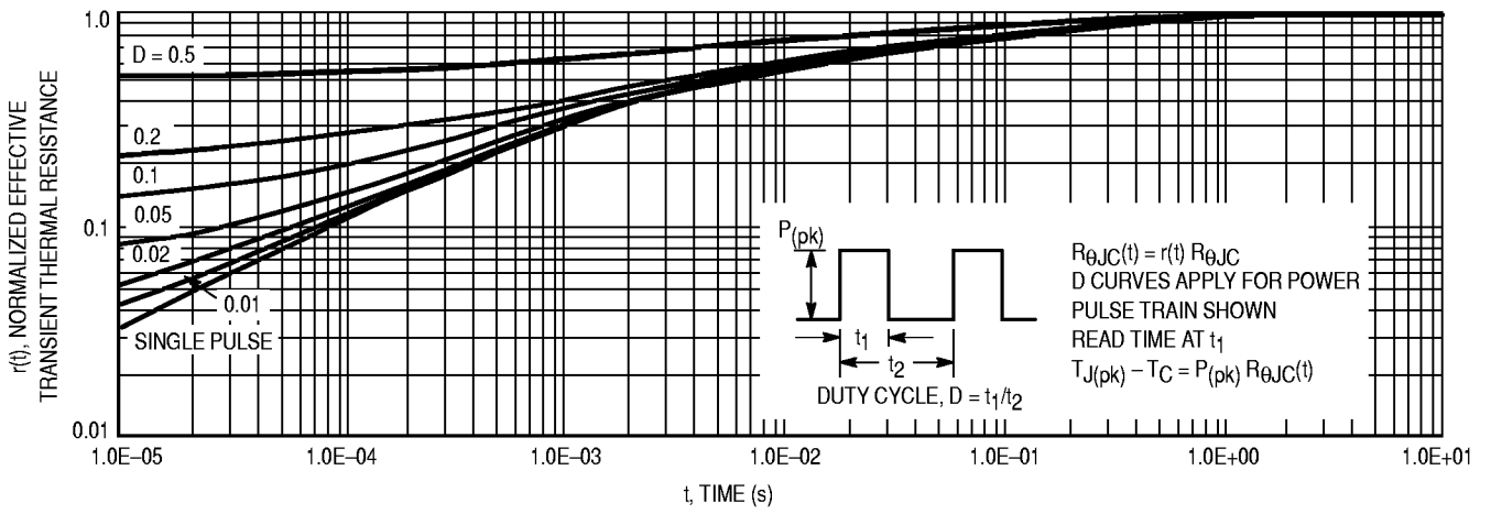
Figure 8. Thermal Response
