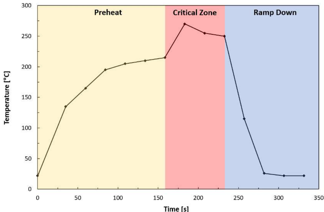
Figure 4. Typical Solder Profile
