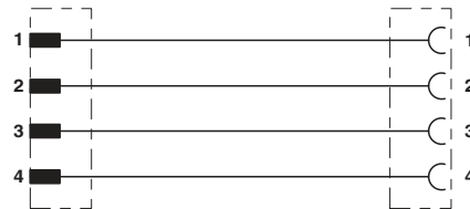
Contact assignment of the DEUTSCH connectors
