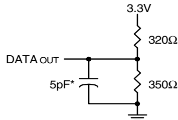
Figure 2. AC Test Load (for t OLZ , t OLZ , t CHZ , t CHZ , t OW , and t WHZ )
