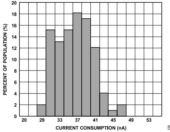
Figure 37. Current Consumption at 25°C, Standby Mode, V_S = 2.1 V
