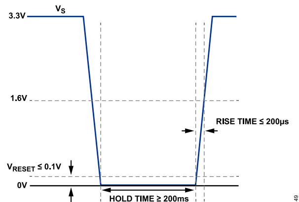
Figure 53. Power Cycling Requirements
