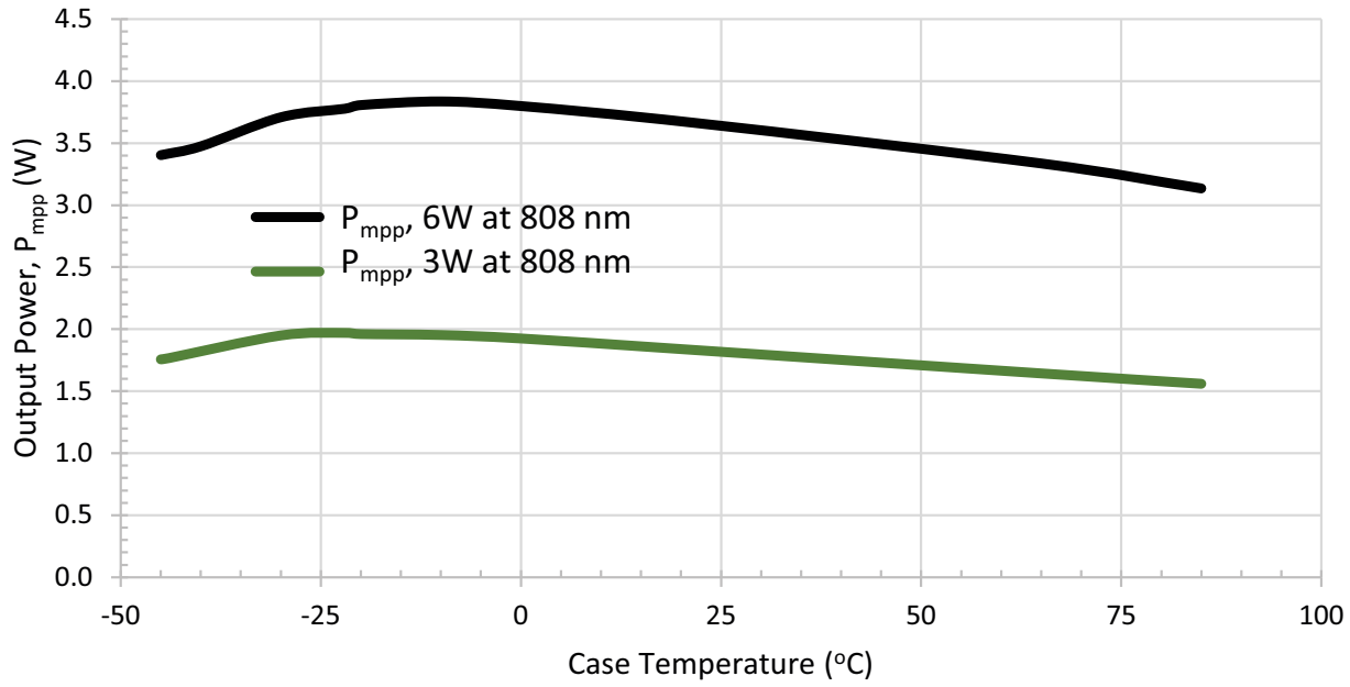
Figure 8: Typical Output Power ( P_{mpp} ) vs. Case Temperature for the AFBR-POC306A1 at 808 nm
