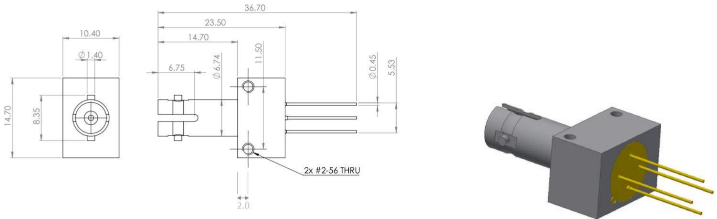
Figure 1: AFBR-POC3xxAx (4 Pins)
