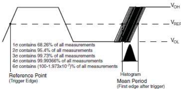
PERIOD JITTER
