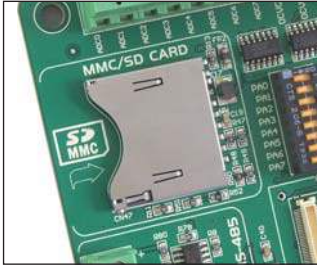
Figure 4-1: MMC/SD connector
