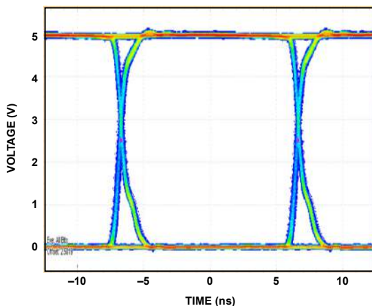
Figure 21. Eye Diagram
