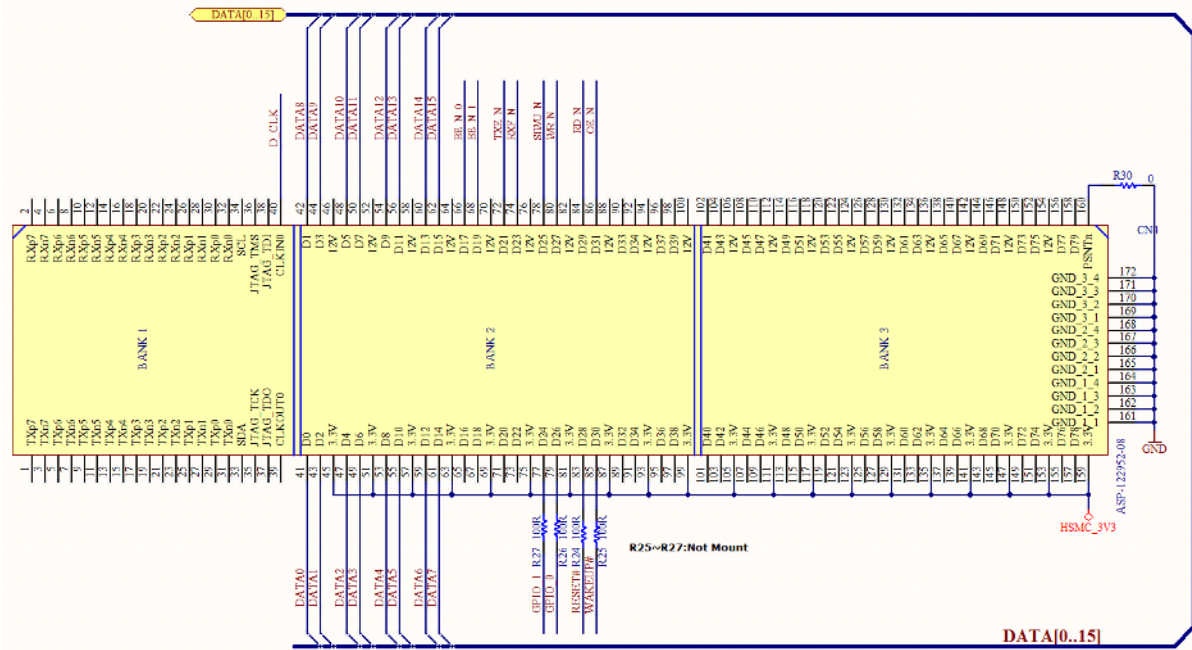
Figure 3-4 Schematics: HSMC_UMFT600A
