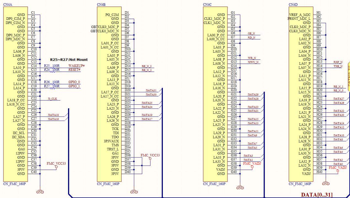
Figure 3-7 Schematics: FMC_UMFT601X
