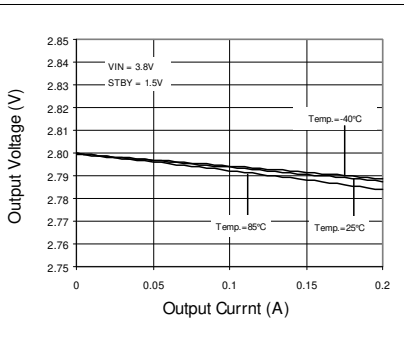
Fig. 98 Load Regulation
