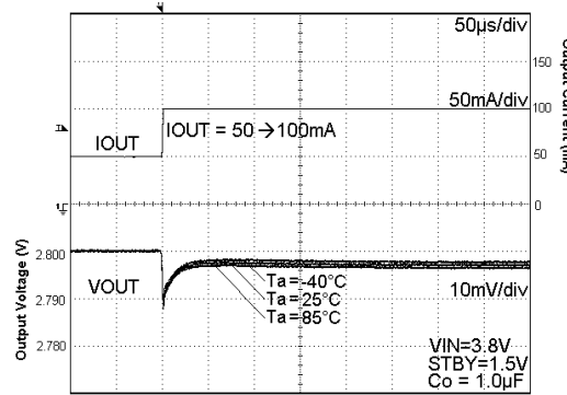
Fig. 109 Load Response
