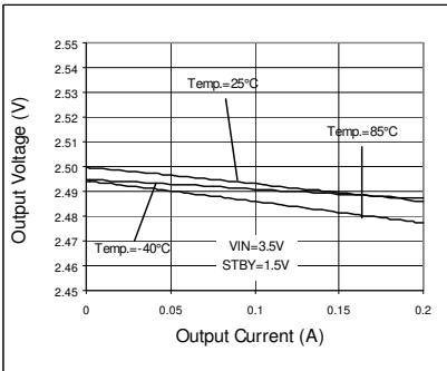
Fig. 69 Load Regulation
