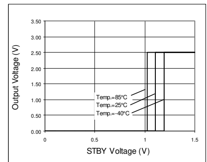
Fig. 71 STBY Threshold
