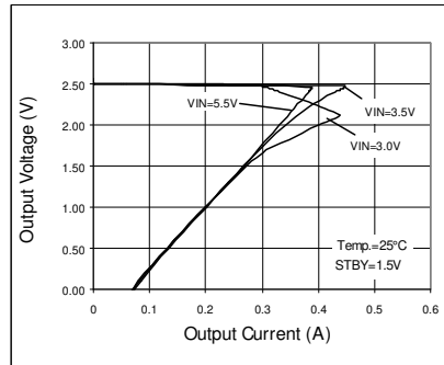
Fig. 70 OCP Threshold
