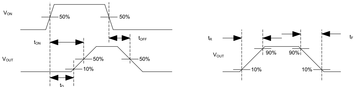
Figure 22. Timing Waveforms
