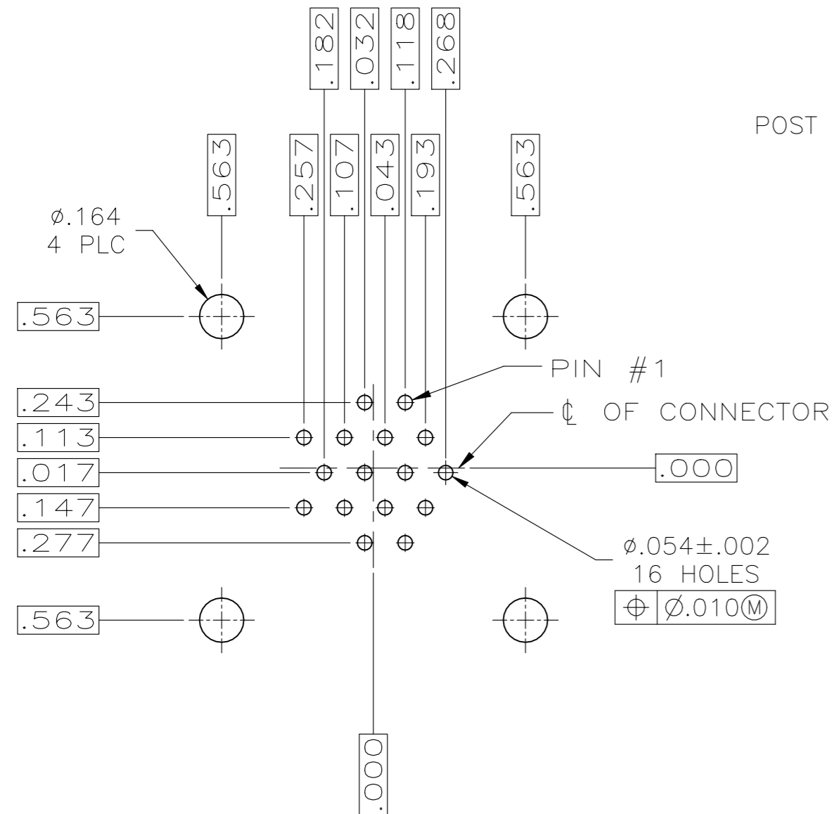
RECOMMENDED P.C. BOARD LAYOUT BOTTOM NON-COMPONENT SIDE
