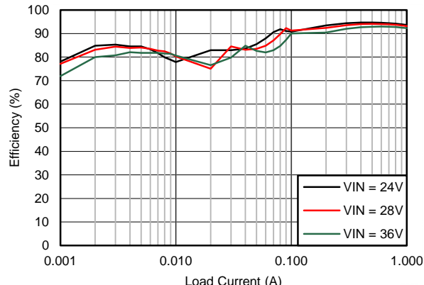
Figure 84. Efficiency
