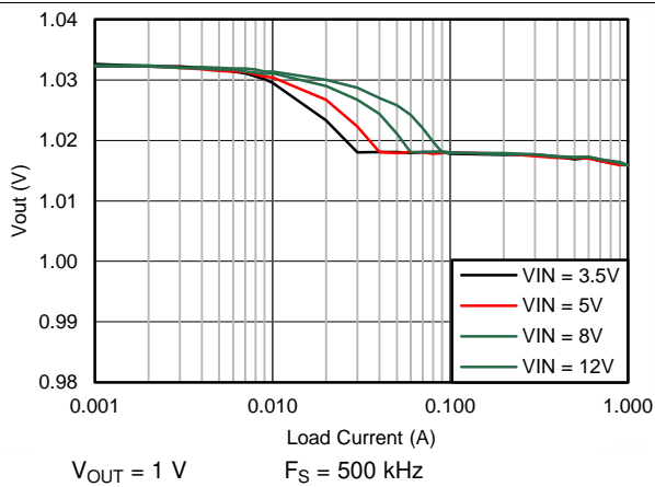
Figure 49. Output Voltage Regulation
