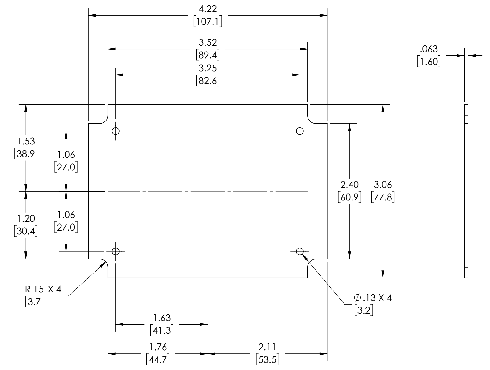
SUGGESTED PCB LAYOUT
