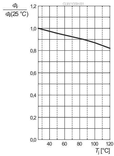
Relative Luminous Flux 6) page 22 Relative Lichtstrom 6) Seite 22 \Phi_V / \Phi_V(25^\circ\text{C}) = f(T_j); I_F = 20 \text{ mA}
