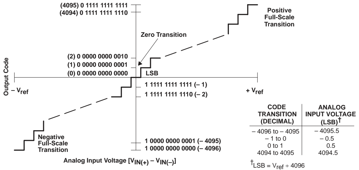
Figure 5. Transfer Characteristic
