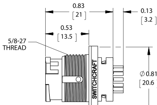
OPTION "C" EN3 SERIES 9-18 POSITION CRIMP TERMINALS EN3P2M26CX SHOWN
