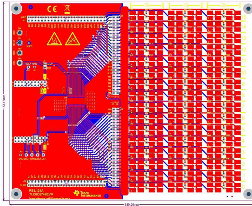
Figure 4-1. TLC6C5748EVM Layout
