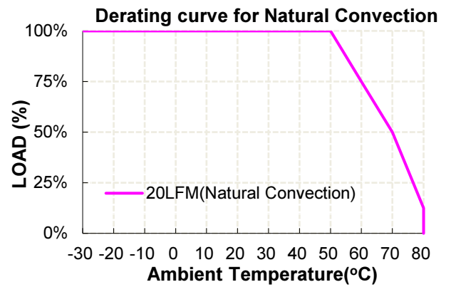
Power Derating
