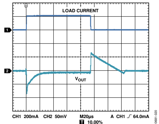
Figure 20. Load Transient Response, C_{IN} = 1\text{ }\mu\text{F} , C_{OUT} = 1\text{ }\mu\text{F} , I_{LOAD} = 1\text{ mA to } 200\text{ mA}
