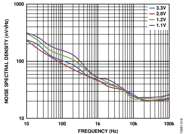
Figure 19. Output Noise Spectral Density vs. Frequency, V_{IN} = 5\text{ V} , I_{LOAD} = 10\text{ mA} , C_{OUT} = 1\text{ }\mu\text{F}
