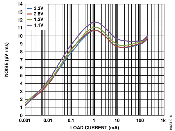
Figure 18. Output Noise vs. Load Current and Output Voltage, V_{IN} = 5\text{ V} , C_{OUT} = 1\text{ }\mu\text{F}
