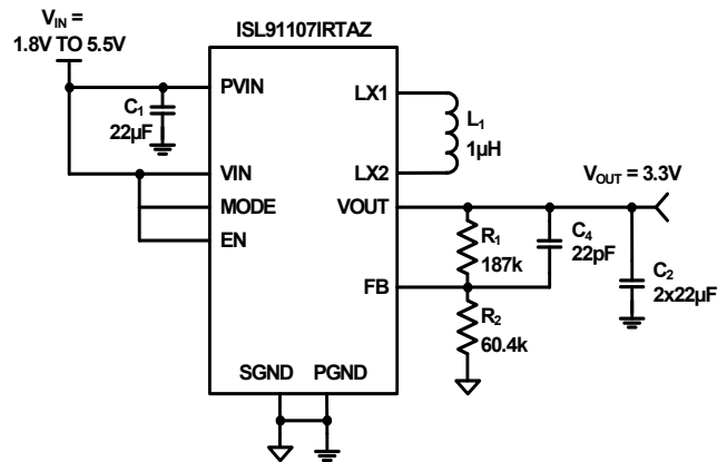
FIGURE 23. TYPICAL APPLICATION
