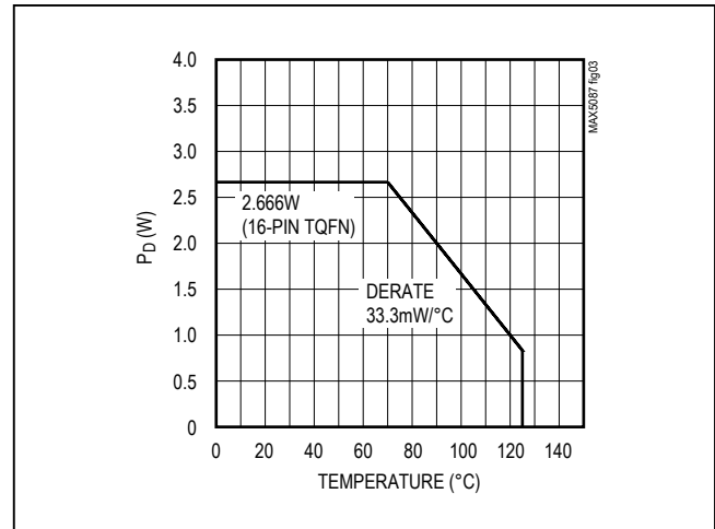
Figure 3. Calculated Maximum Power Dissipation vs. Temperature
