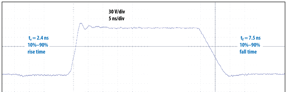
Waveform 8 A, V_{IN} = 160\text{ V} , V_{OUT} = 28\text{ V} , L = 200\text{ kHz}
