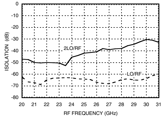
LO/RF Isolations
