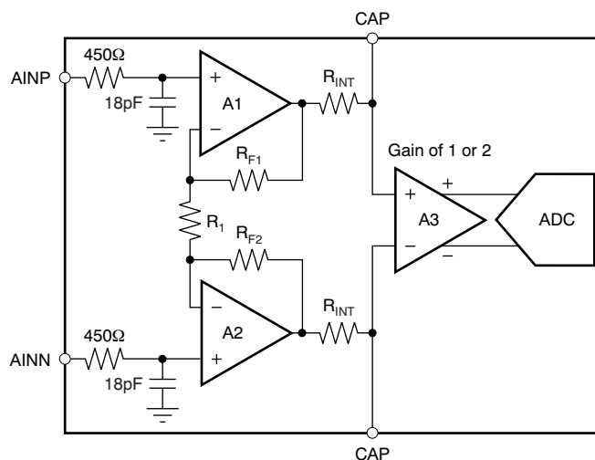
Figure 8-2. Simplified Diagram of the PGA
