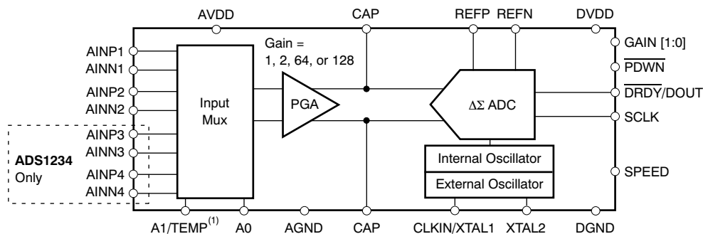
Block Diagram
