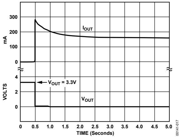
Figure 17. Short-Circuit Current
