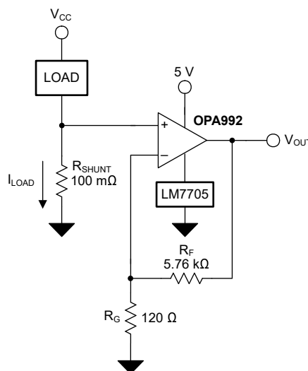
Figure 8-1. OPAx992 in a Low-Side, Current-Sensing Application
