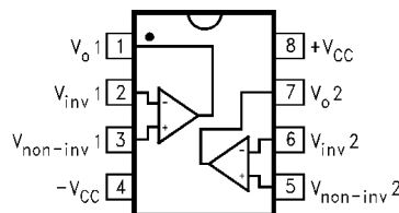
Pinout DIP & SOIC
