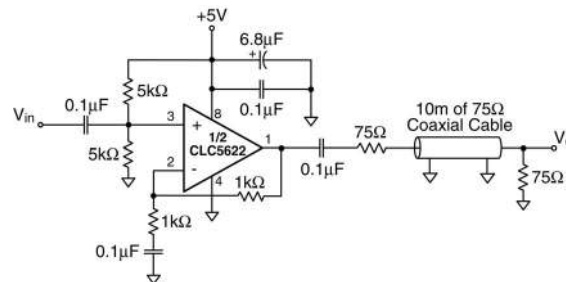
FIGURE 10. Single Supply Cable Driver
