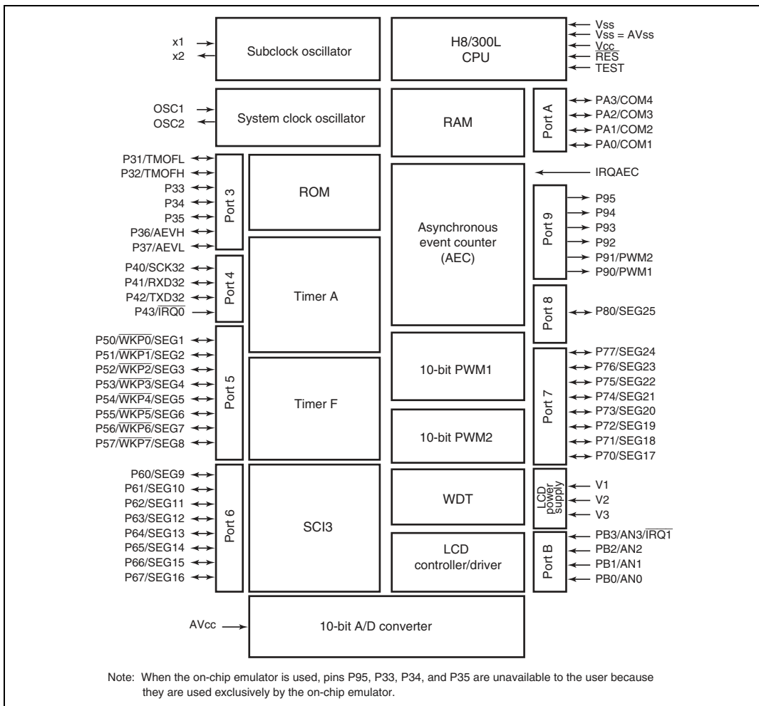
Figure 1.2 Internal Block Diagram of H8/38004 and H8/38002S Group
