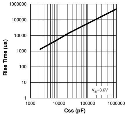
VOUT Rise Time vs Coss
