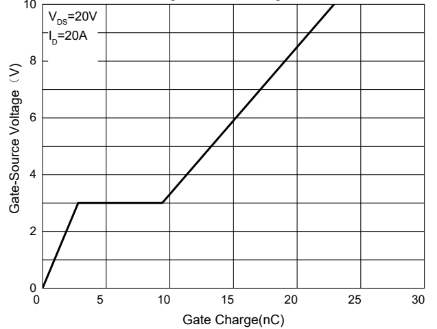
Fig. 6 - Gate Charge
