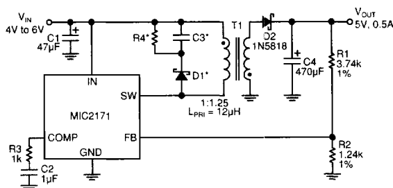
Figure 2. MIC2171 5V Flyback Converter
