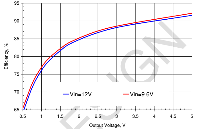
Figure 3. Efficiency vs. Output Voltage, Iout=10A
