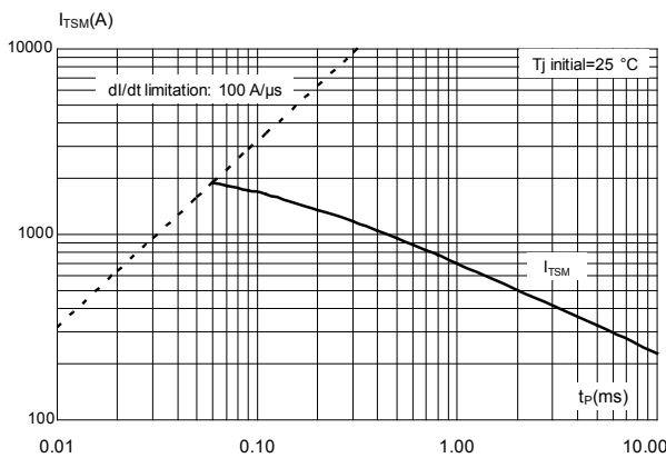
Figure 7. Non-repetitive surge peak on-state current for a sinusoidal pulse
