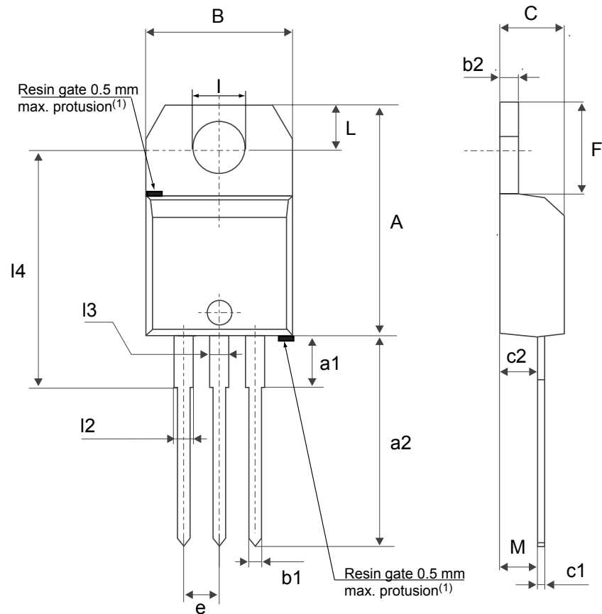
Figure 16. TO-220AB package outline
