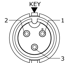
FACE VIEW 6282-3PG-5XXW
