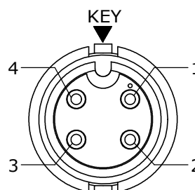
FACE VIEW 6282-4PG-5XXW
