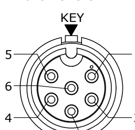
FACE VIEW 6282-6PG-5XXW
