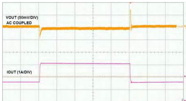
Time- 200µs/div Load Transient Test I_{OUT} = 1.5A \text{ to } 3A . Step at 0.8A/\mu s
