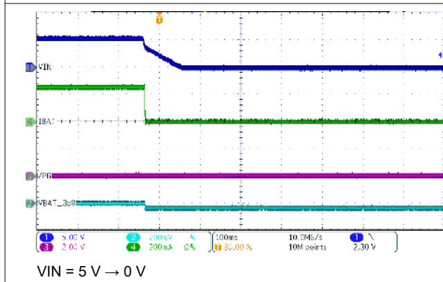
Figure 8-4. Power Down
