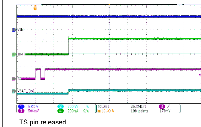
Figure 8-6. Charge Enable
