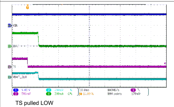
Figure 8-5. Charge Disable
