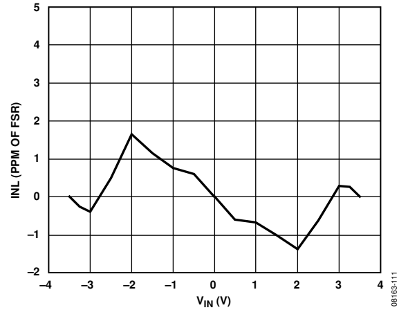
Figure 11. INL (Gain = 1)
