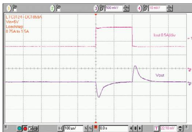
Figure 4. The LTC3124 Has Excellent Load Step Response with Small Output Capacitors Thanks to High Switching Frequency and Fast Feedback Loop Compensation
