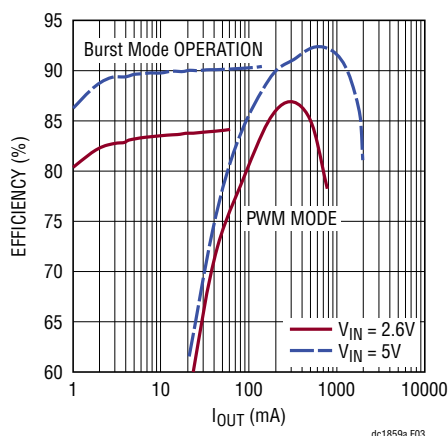
Figure 3. The Efficiency Is Maximized for Light Loads by Shedding One Phase in Burst Mode Operation. The Efficiency Is Over 90% at Higher Loads and It Reaches 92% at 800mA Load
