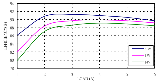
Figure 4: Converter efficiency vs. output current (1.8V output voltage)
