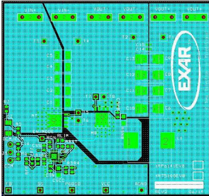
Fig. 3: Component Placement – Top Side
