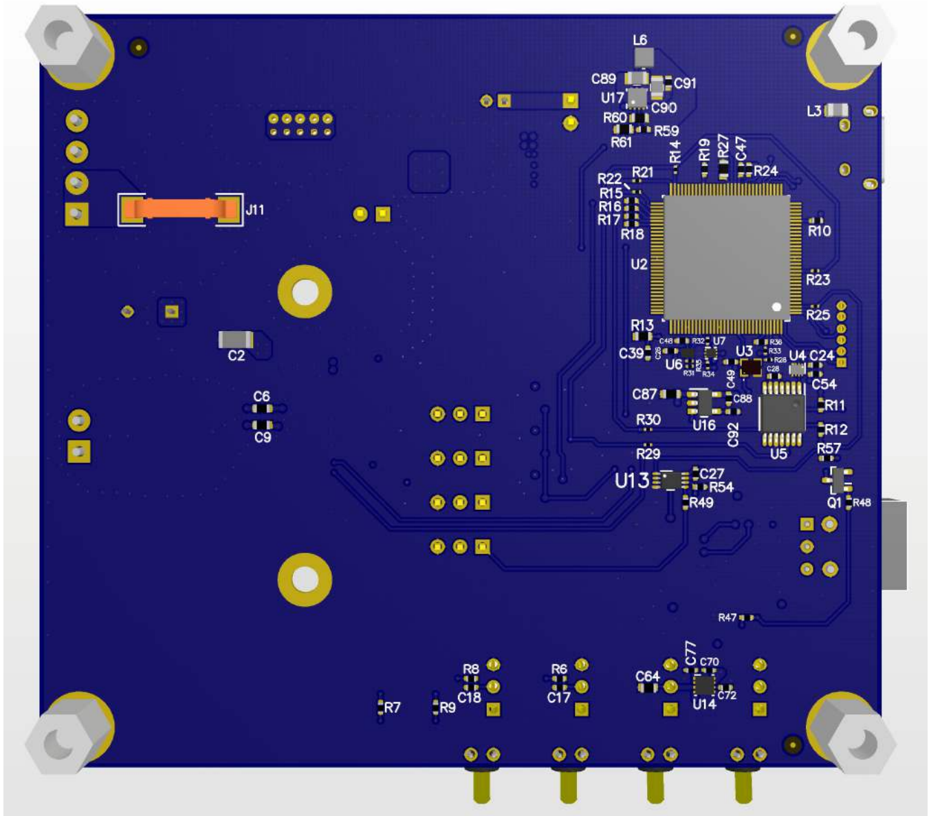
Figure 21. TAS6421-Q1 EVM Bottom
