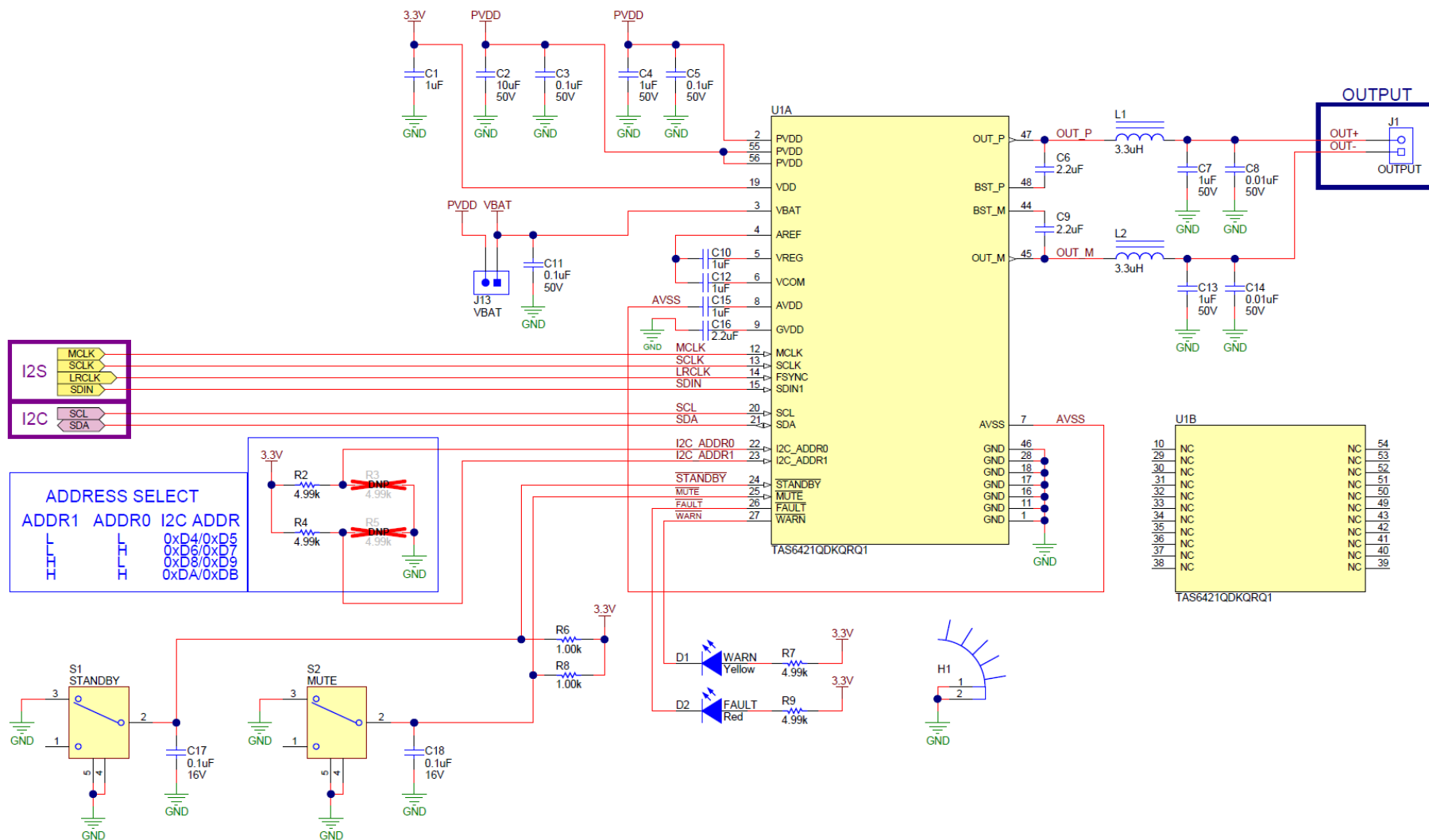
Figure 24. Schematic (Page 3)
