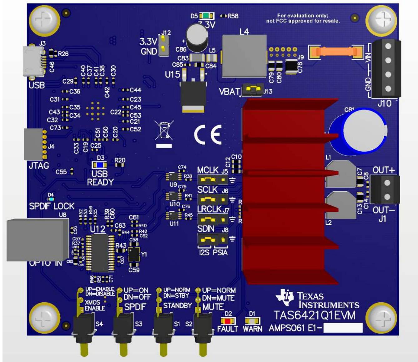
Figure 20. TAS6421-Q1 EVM Top
