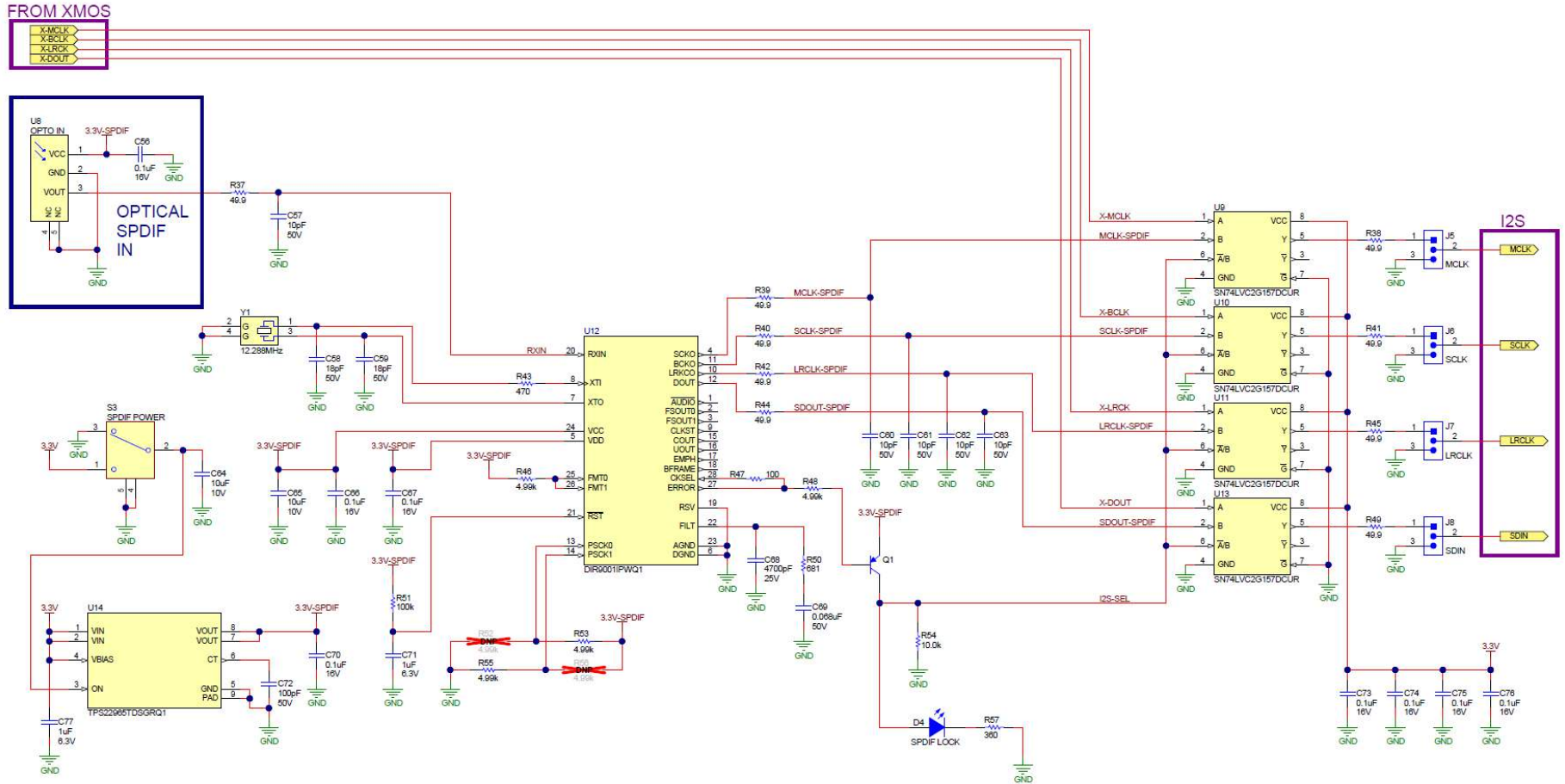
Figure 23. Schematic (Page 2)
