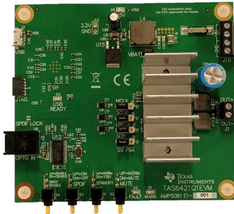
Figure 1. TAS6421-Q1 EVM
