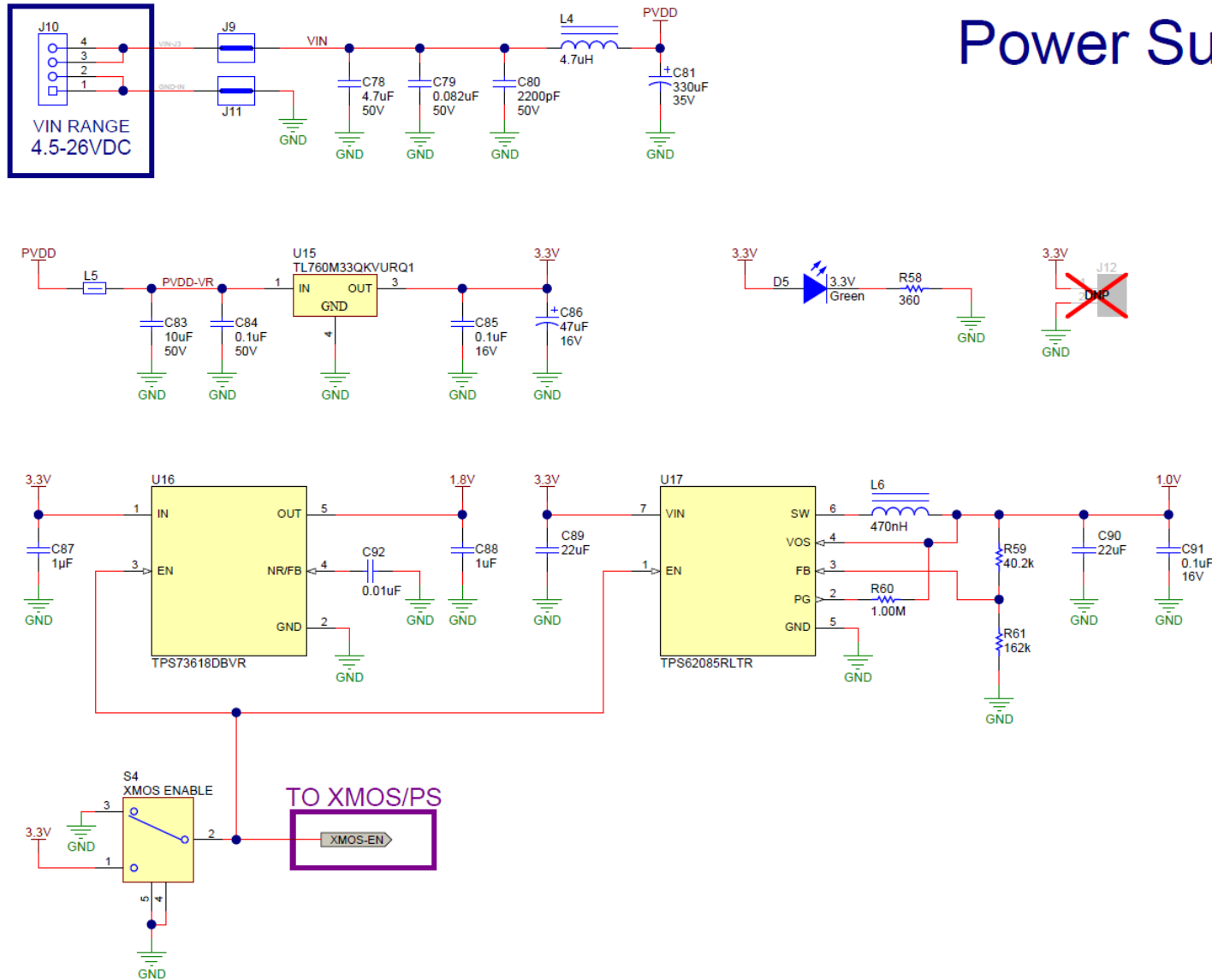
Figure 25. Schematic (Page 4)
