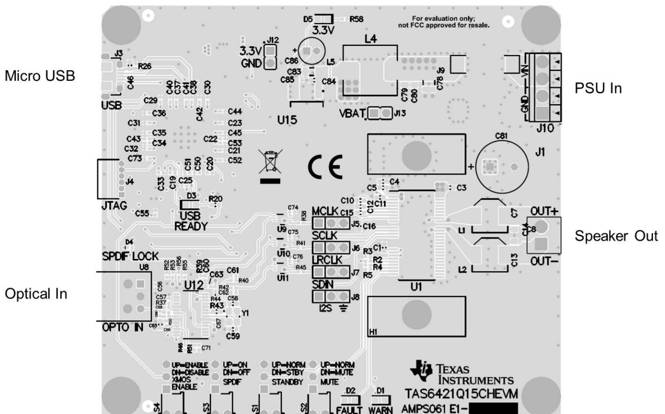
Figure 8. TAS6421-Q1 EVM Connections
