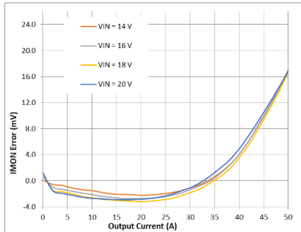
Figure 25. I_{MON} Accuracy vs. Input Voltage
